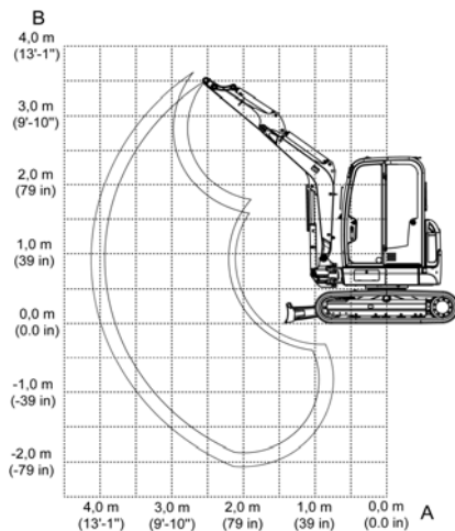
Fig. 1: Lifting force table EZ28
